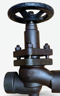
Piston Valve Screw End MOC: C.S. Range: 15mm to 50mm
