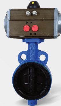
Butterfly Valve with Actuator MOC: C.I. / C.S. / S.S Range: 40mm to 300mm
