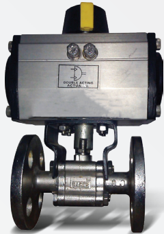
IC Actuator Ball Valve MOC: CF8 / CF8M Range: 15mm to 200mm
